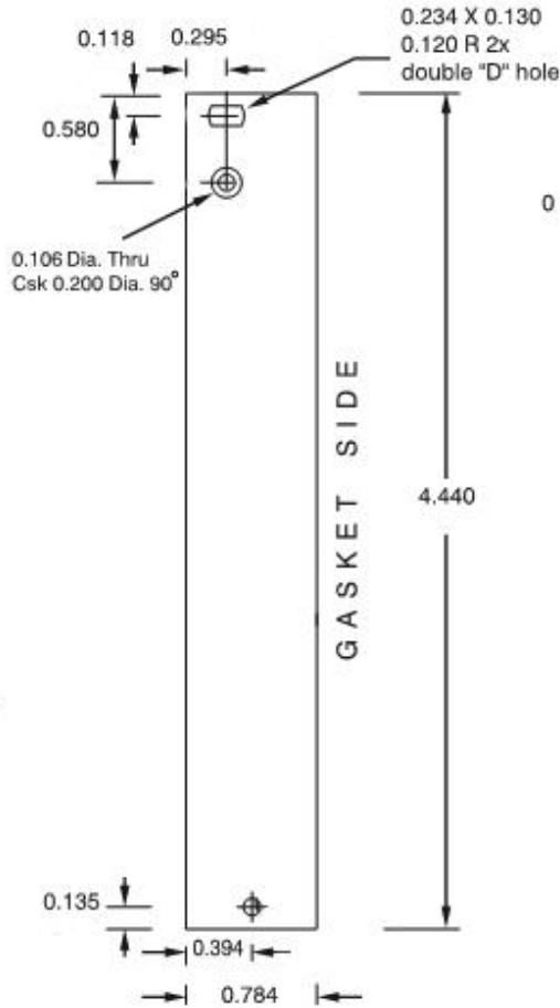
cPCI 3U x 4HP
